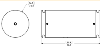
Electronics Housing
